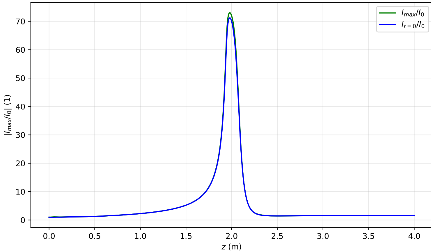
I_{max}(x=0, y=0, z)/I_0 , P_{in}=1.4P_{cr} , noisy input, artificial time
